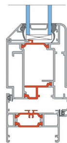
Cill Detail
